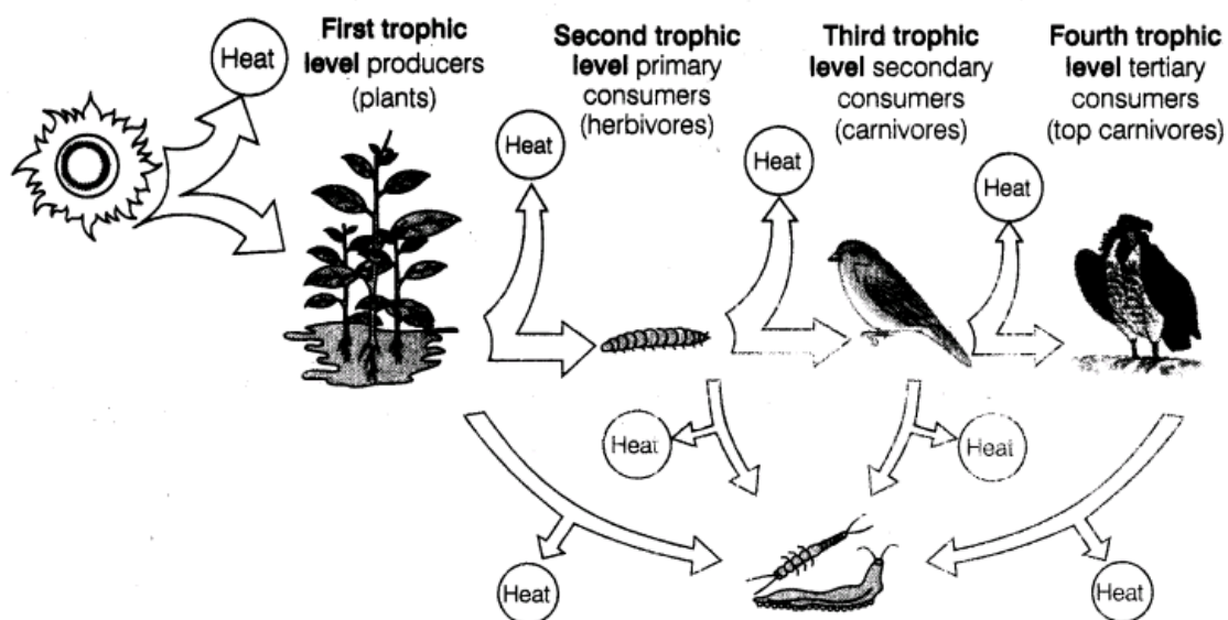
Diagrammatic representation of flow of energy through different trophic levels
